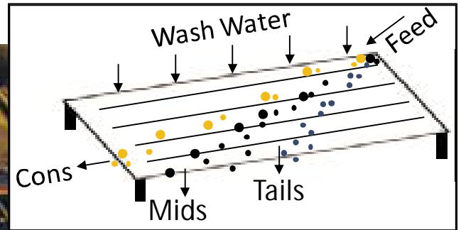
schematic of a shaking table
