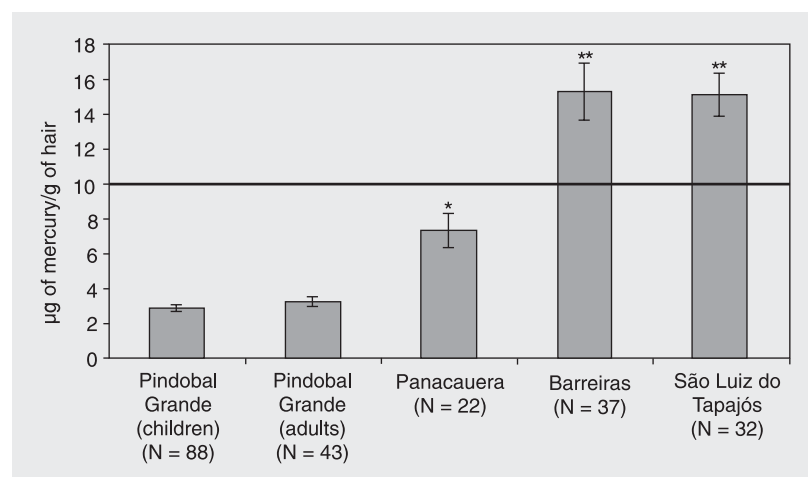
Figure 2. Total mercury content in hair samples from 2 regions of the Amazon. Data are reported as mean \pm SEM. The horizontal line at 10 \mu\text{g/g} indicates the limit determined by the World Health Organization. ** P < 0.001 vs Panacauera and Pindobal Grande (adults and children); * P < 0.05 vs Pindobal Grande (adults and children; Tukey post hoc test).
